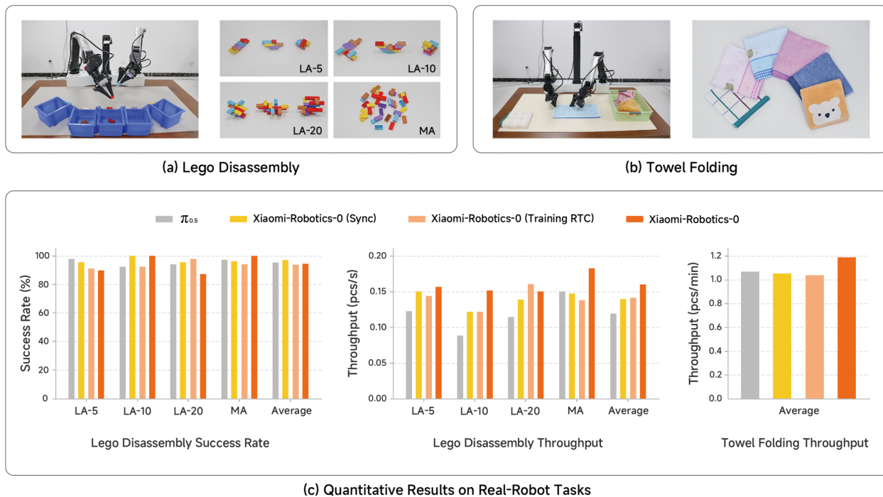
Figure 6 Real-Robot Experiments. (a) We show the setting for Lego Disassembly evaluation. (b) We show the setting for Towel Folding evaluation and all the towels used during evaluation. (c) Quantitative results of different methods on the two tasks.
