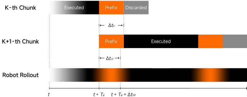
Figure 5 Asynchronous Execution. We show two consecutive chunks and how they are stitched together during robot rollout. See Sec. 2.3 for more details.
